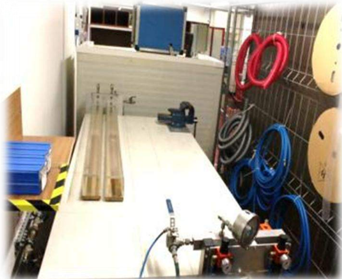
Hose Testing Machine Prima Design
